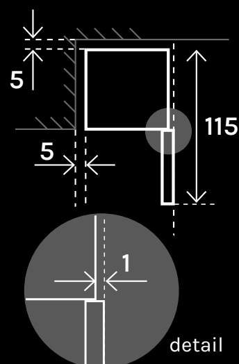
Doors opening dimensions (cm)
